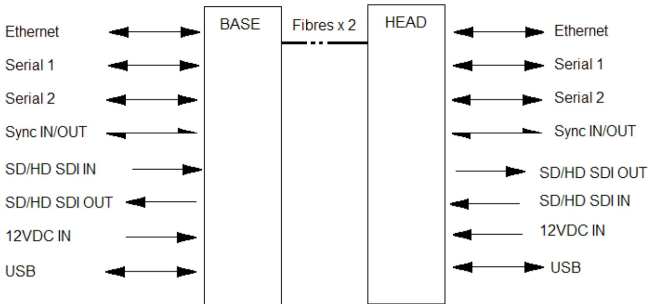
CAMLINX Zero : Block diagram
