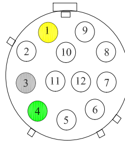
OUTSIDE VIEW
